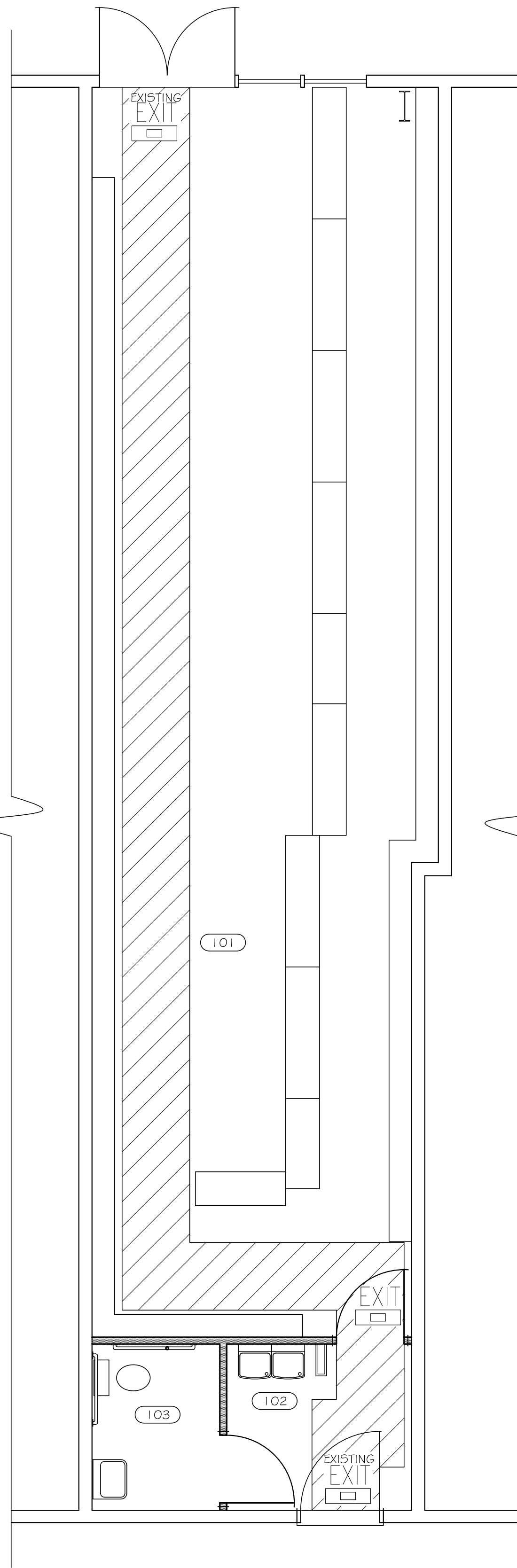
FIRST FLOOR EGRESS PLAN SCALE: 1/4" = 1'-0"
