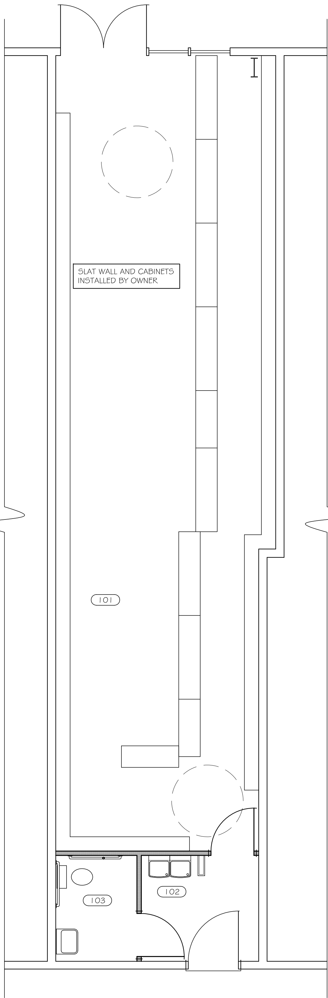
FIRST FLOOR FIXTURE PLAN SCALE: 1/4" = 1'-0"
