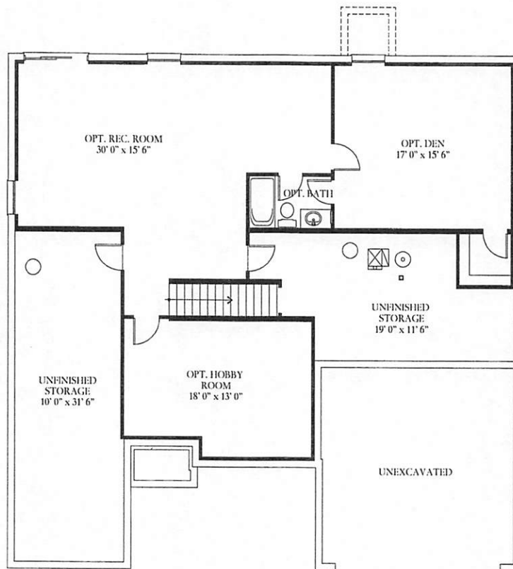
Unfinished Basement
