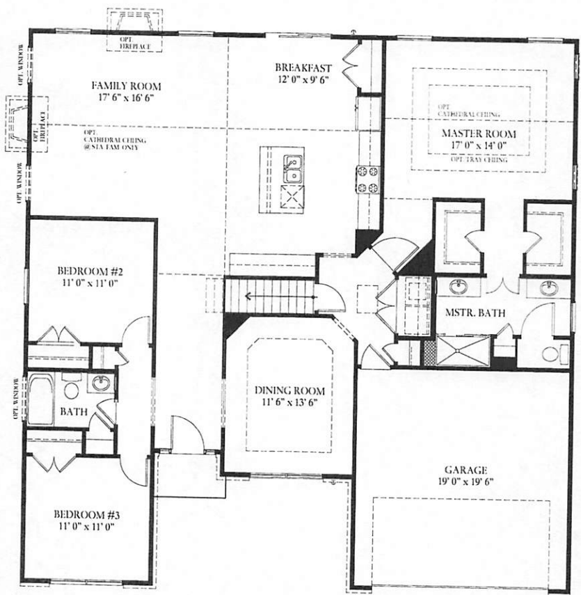
Ext. Family & Morning Rooms
