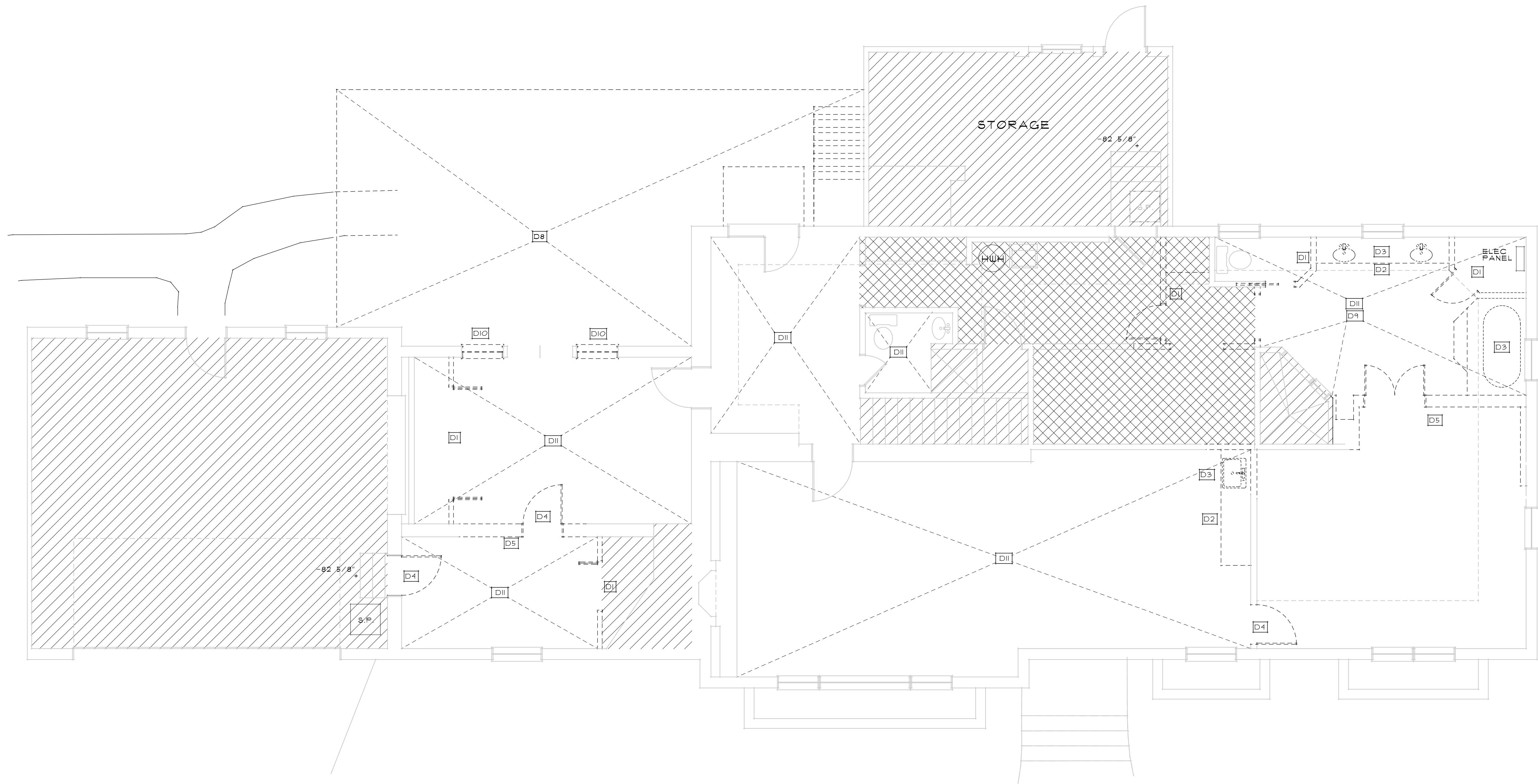
1 BASEMENT DEMOLITION PLAN SCALE : 1/4" = 1'-0"
