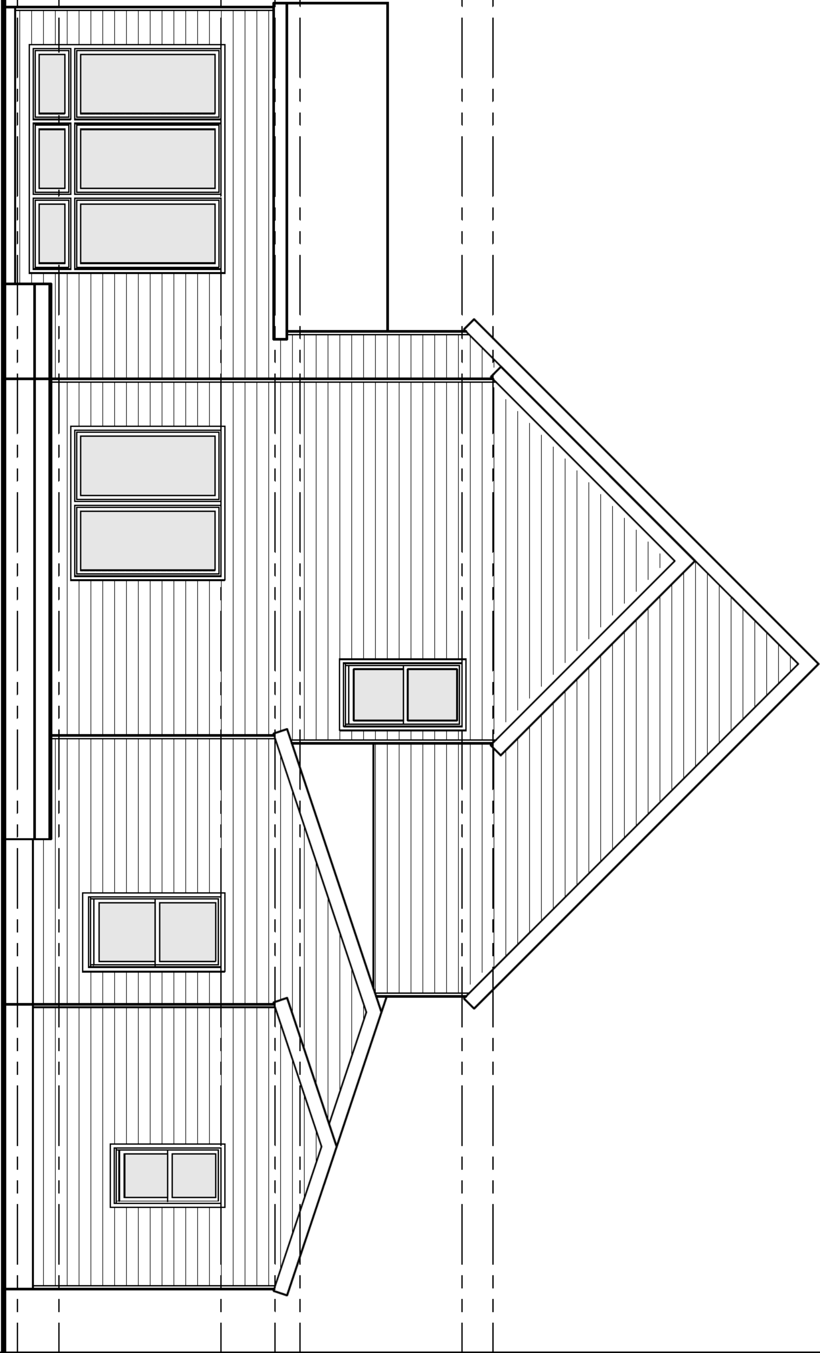
REAR ELEVATION
