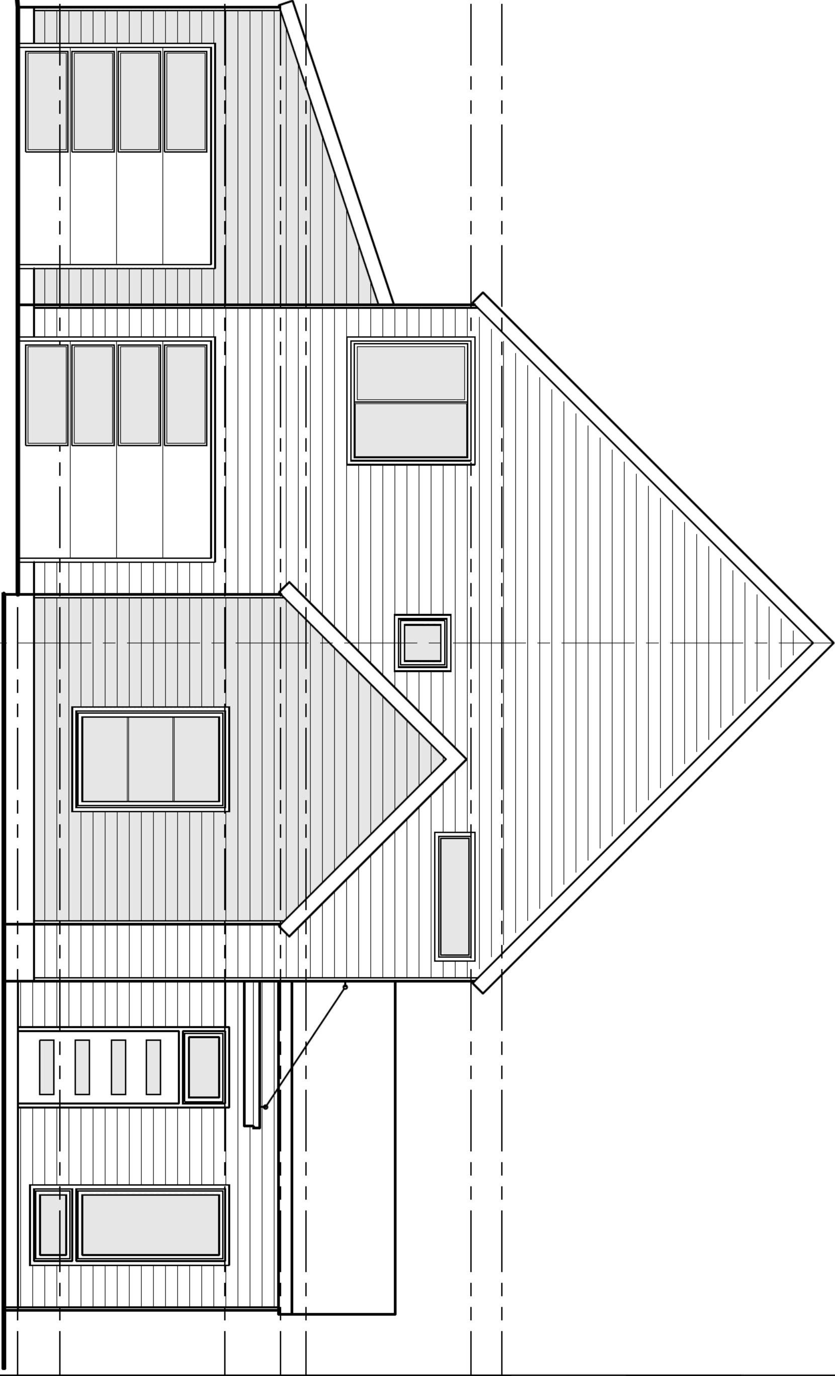
FRONT ELEVATION
