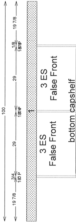
Plan View Rolling Cart
